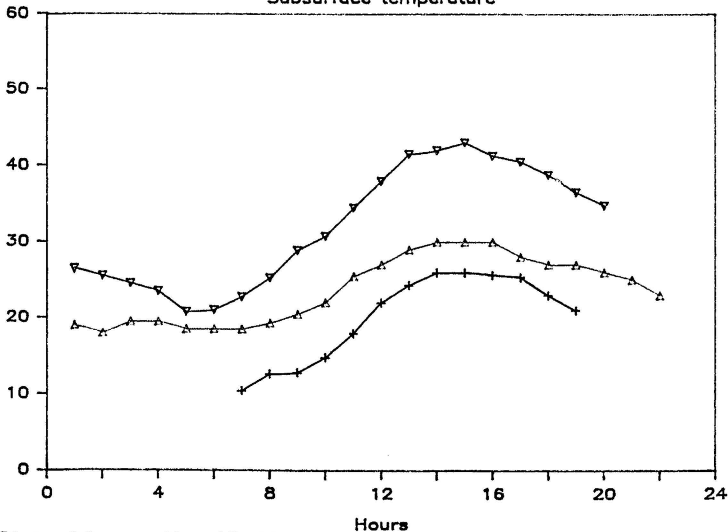
Subsurface temperature
