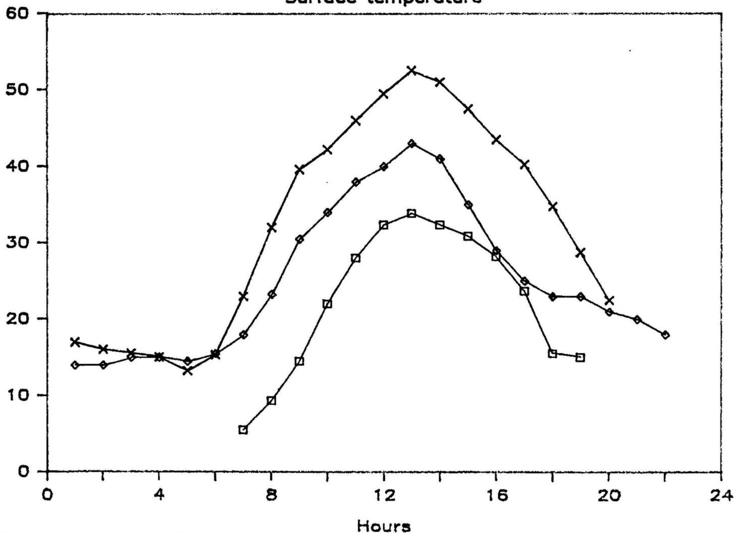
Surface temperature
